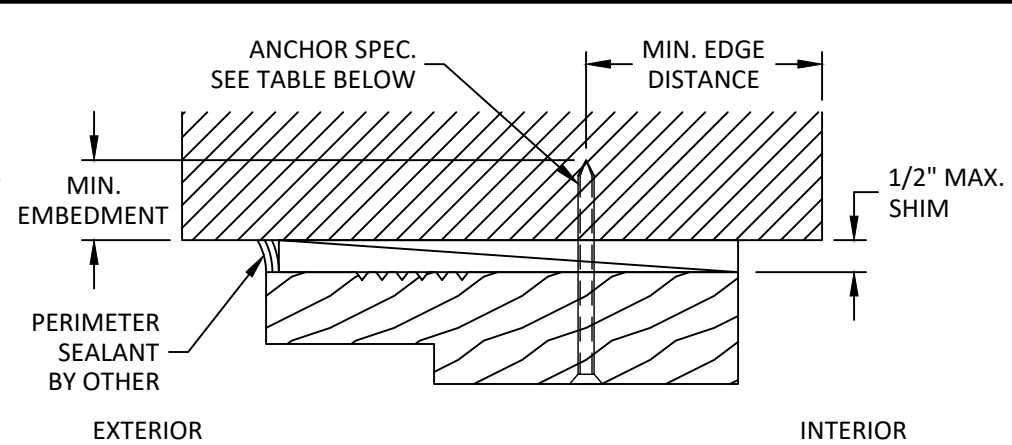
R 16 INSTALLATION DETAIL SIDELITE/TRANSOM HEAD HEAD SHOWN, JAMB & SILL SIMILAR
