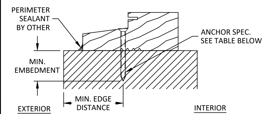
T 16 INSTALLATION DETAIL OUTSWING DOOR SILL
