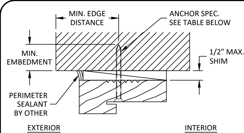
Q 16 INSTALLATION DETAIL DOOR HEAD HEAD SHOWN, JAMB SIMILAR INSWING SHOWN, OUTSWING SIMILAR
