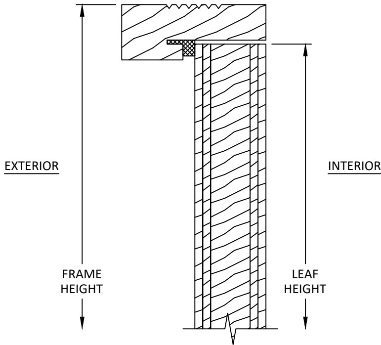
A 12 VERTICAL SECTION INSWING DOOR HEAD
