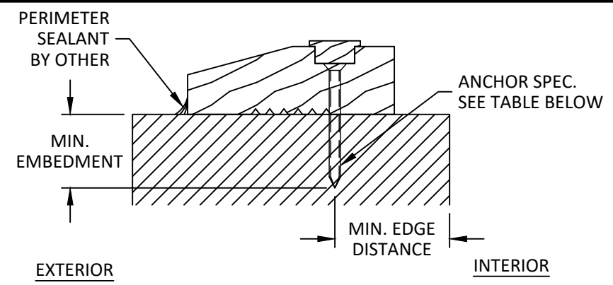
S 16 INSTALLATION DETAIL INSWING DOOR SILL
