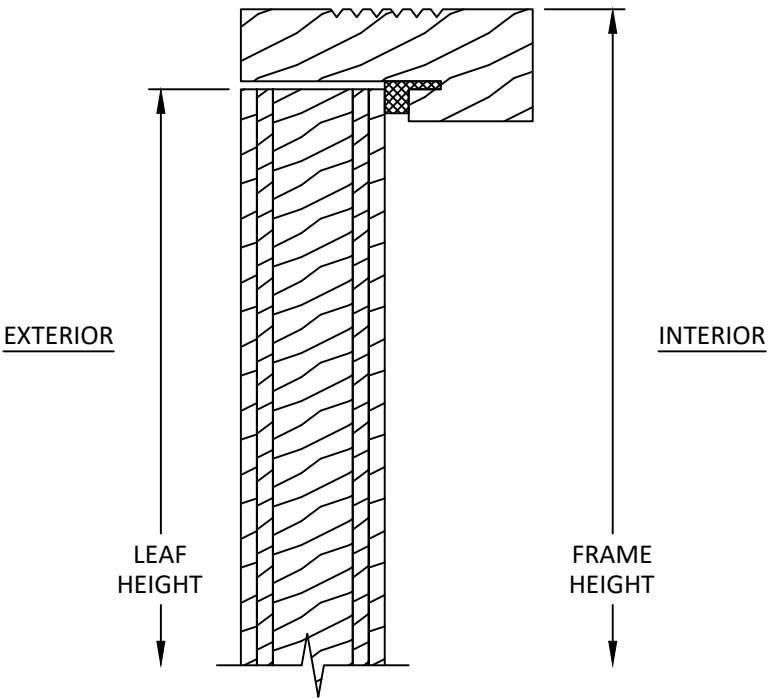
C 12 VERTICAL SECTION OUTSWING DOOR HEAD
